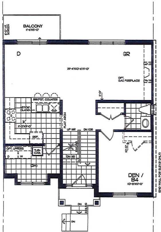
MAIN FLOOR - ELEV. A/B
